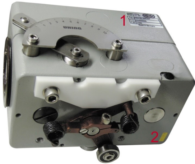
Illustration 5: Rolling Ring Drive RG3/4-50-0...-RG3/4-80-0...
